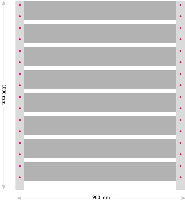
FIGURE 1: SIDE PANEL CONSTRUCTION
