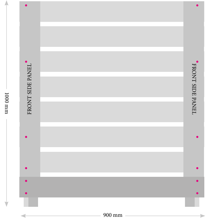
FIGURE 2: FRONT VIEW (WITHOUT FRONT SLATS)
